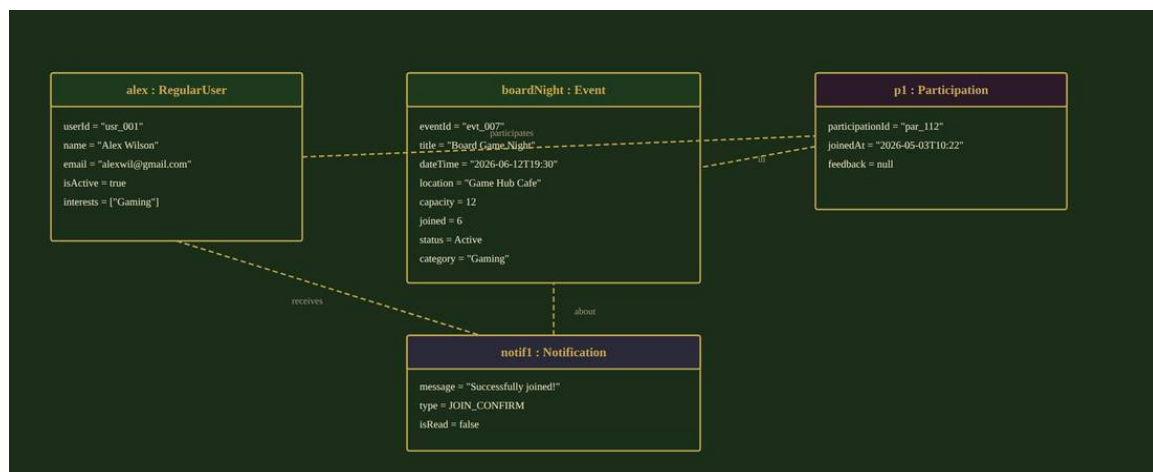
Figure 3.3 – Object Diagram – “Join Event” snapshot
