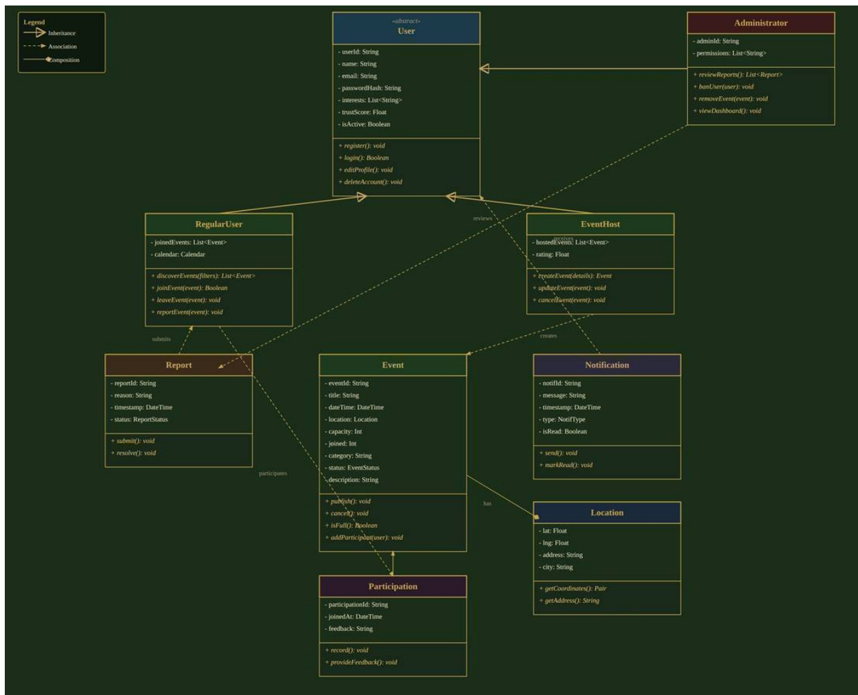
Figure 3.2 – LoneWolf Class Diagram
